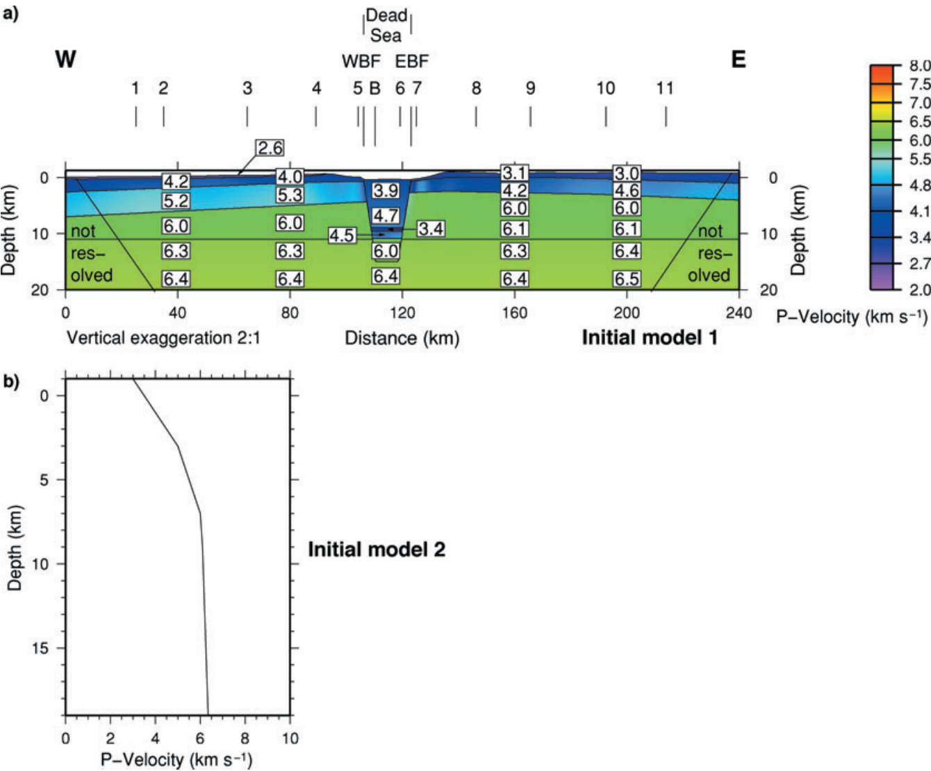
Figure 10. (a) Two-dimensional initial P -wave velocity model (velocities in km s -1 ) for the inversion, which produced the model shown in Fig. 11(a). (b) 1-D initial P -wave velocity model for the tomography that produced the upper crustal part of the model shown in Fig. 11b. The positions of the shotpoints are marked above the 2-D model. Key: WBF: Western Boundary Fault, EBF: Eastern Boundary Fault, B: international boundary.
