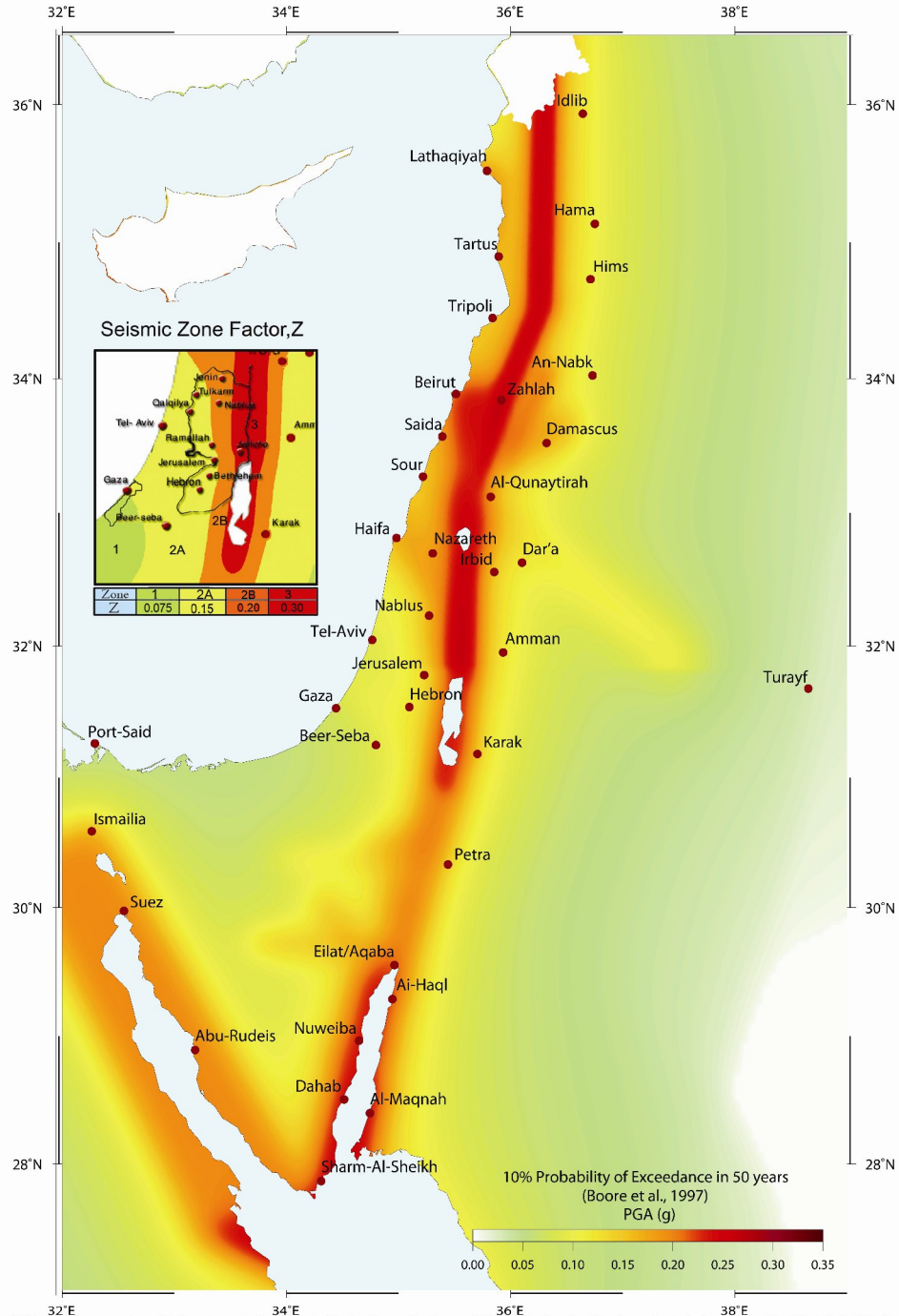
Appendix 1.1 -a: Seismic Hazard Map /Peak Ground Acceleration Map (PGA map) and Seismic Zone Factor (Source ESSEC)
