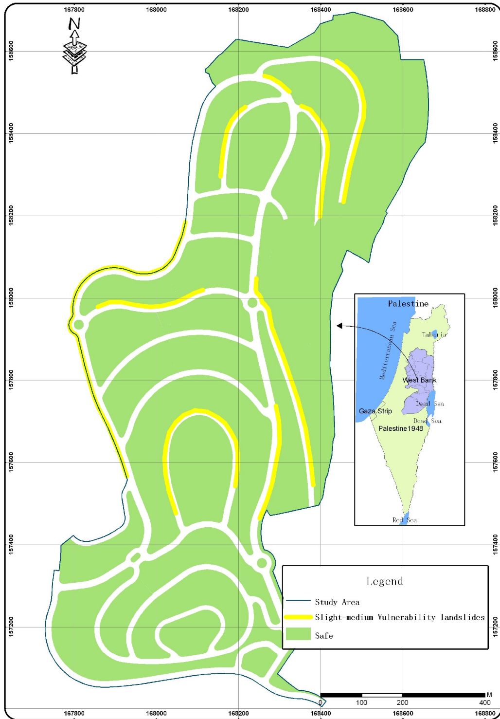
Appendix 5.2: Landslides map.
